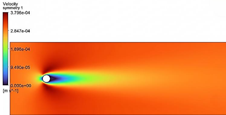
Figure 2. Velocity magnitude contour for Re = 20 (Steady Laminar Flow). The wake is symmetric and no vortex shedding is observed. Max velocity: 3.796 \times 10^{-4} m/s
